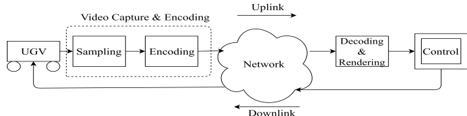
Fig. 1: Block diagram for communication between UGV and command center.
