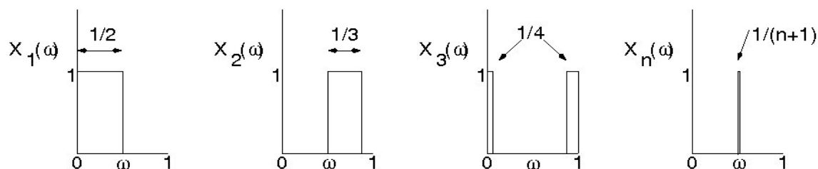
Figure 1.2: The random variables X_1, X_2, \dots , in Example 1.9.
