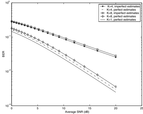
Fig. 1. BER performance of the decorrelating detector without and with channel estimation errors for K = 4, 8, L = 1 .
