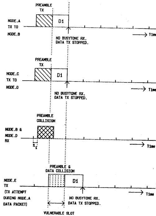
FIG. 4. Illustration of preamble collision in slot ' n ' & new tx. attempt in vulnerable slot(s) ' n+k '. ( k=1 )
