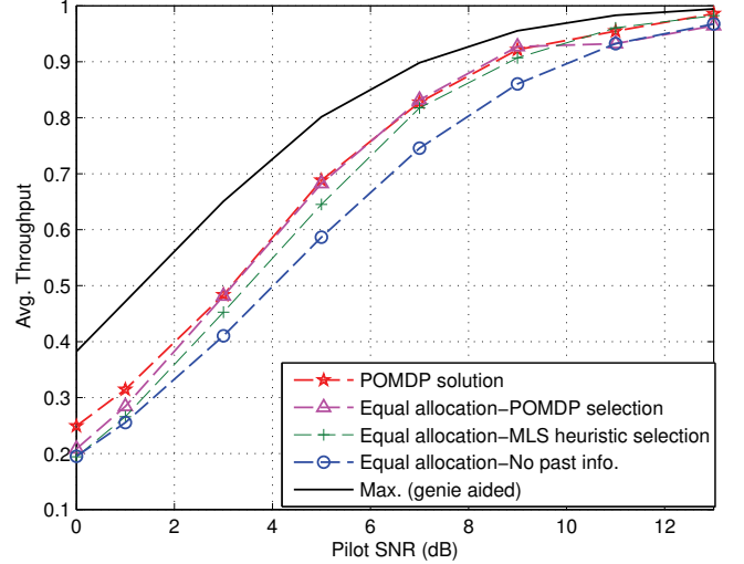
Fig. 5. Avg. throughput vs. pilot SNR for FSMC model ( N = 4 , L = 4 , G = 4 , data SNR = pilot SNR - 3 dB, f_d T_f = 0.01 ).
