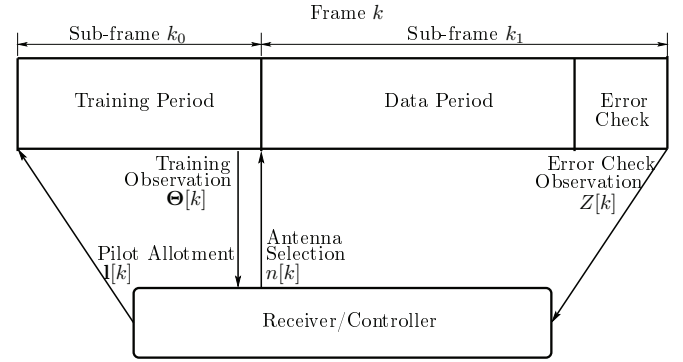
Fig. 3. Sequence of operations in frame k .
