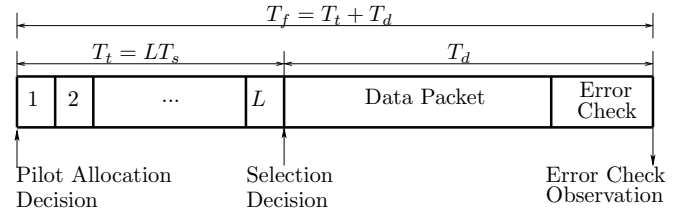
Fig. 1. Frame structure for training and data reception.
