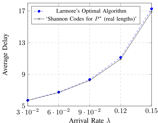
(a) Comparison of proposed codes with Larmore's Algorithms [16] for the distribution P(1) = 0.5 , and P(i) = \frac{0.5}{255} \quad \forall i \in \{2, \dots, 256\} .
