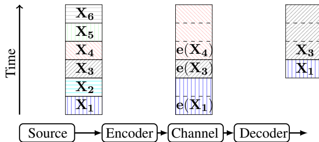
Fig. 1: An example of the proposed memoryless update scheme, where the symbol X_2 is skipped since the channel was busy sending X_1 when it arrived. Furthermore, the decoder retains output X_3 , a symbol which was received within a delay of 1 time unit, for 3 time slots while X_4 was being sent.
