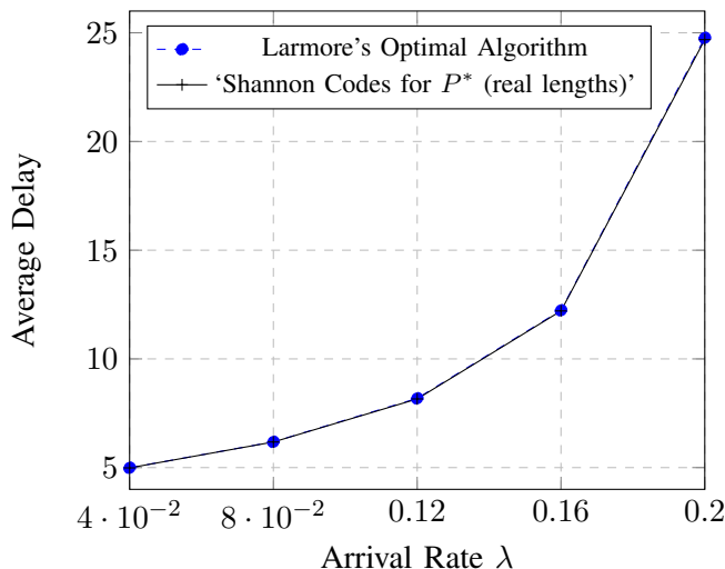
(b) Comparison of proposed codes with Larmore's Algorithms [16] for the distribution P(1) = 0.6 , and P(i) = \frac{0.4}{255} \quad \forall i \in \{2, \dots, 256\} .
