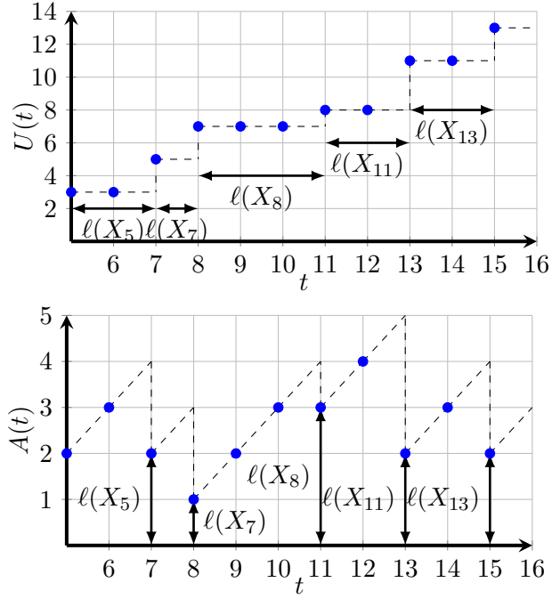
Fig. 2: A sample path of U(t) , A(t) with U(5) = 3 .
