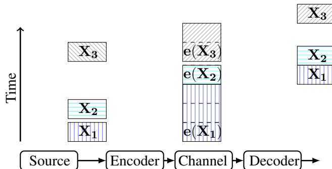
Fig. 6: Figure describes a typical sample-path for transmission of encoded symbols over a FCFS queuing system. Symbol X_1 arrives at some time instant 1, it is encoded and transmitted over the channel. It is decoded at time instant 4. Symbol X_2 arrives in between time instants 2 and 3, and is placed in the queue, as the channel is busy transmitting X_1 . As soon as the channel becomes free at time slot 4, an encoded version of X_2 is transmitted over it. Symbol X_3 arrives when the channel is free and is transmitted immediately.
