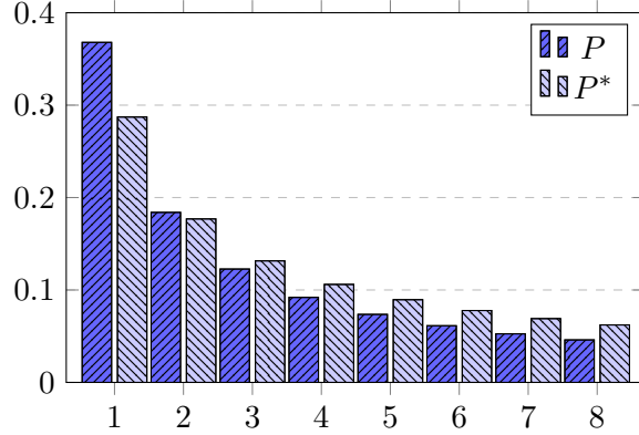
Fig. 4: Pmf for P^* and P for \text{Zipf}(1, 8) .
