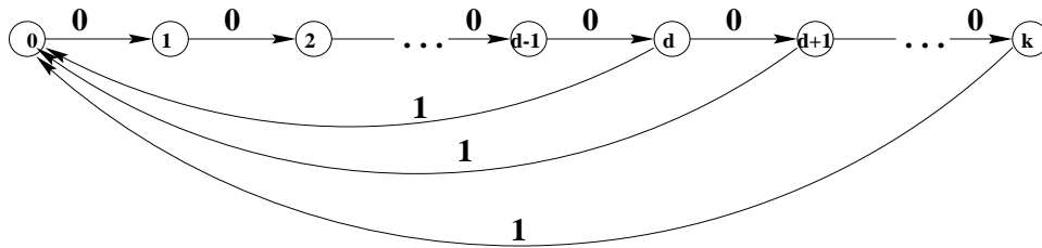
Fig. 1. Graph, \mathcal{G}_{d,k} , generating the (d,k) -constrained system \mathcal{S}(d,k) for finite k .
