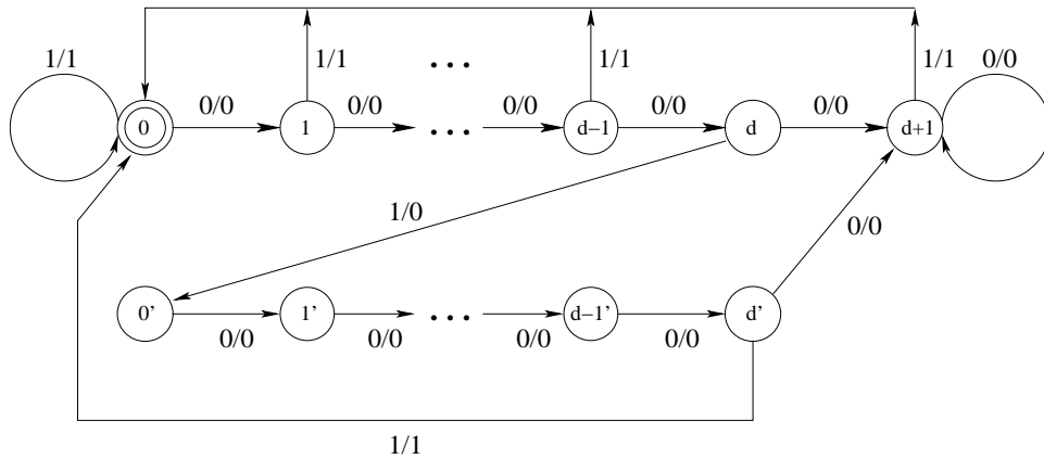
Fig. 4. Encoder from \mathcal{S}(d, 2d) to \mathcal{S}(d+1, 3d+1) .
