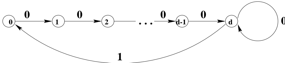
Fig. 2. Graph, \mathcal{G}_{d,\infty} , generating the (d,\infty) -constrained system \mathcal{S}(d,\infty) .
