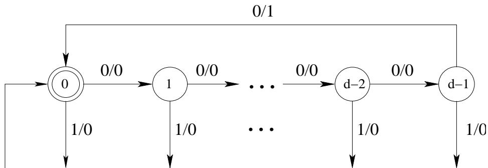
Fig. 5. Encoder from \mathcal{S}(d, \infty) to \mathcal{S}(d-1, 2d-1) .
