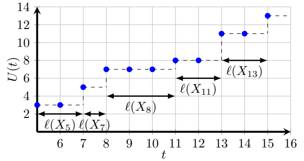
Fig. 2: A sample path of U(t) with U(5) = 3 .
