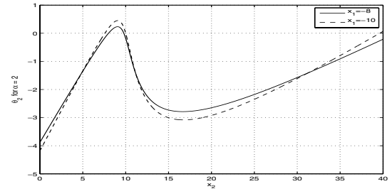
Fig. 2. Single-frequency case; fixed BS locations at x_1 and x_2 : Upper cell boundary of cell A_1 (vertical axis) as a function of the location of BS 2 (horizontal axis) for various locations of BS 1.
