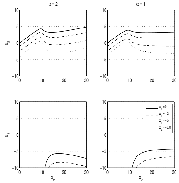
Fig. 1. Single-frequency case; fixed BS locations at x_1 and x_2 : Thresholds determining the cell boundaries (vertical axis) as a function of the location of BS 2 (horizontal axis) for various locations of BS 1. The path loss exponent \alpha is 2 in the figures on the left and 1 in those on the right.
