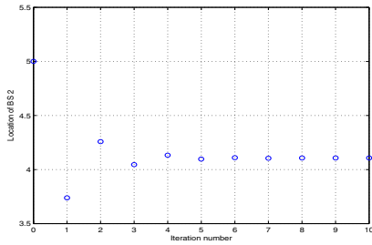
Fig. 8. Two frequencies case; non-cooperative BSs: Convergence to equilibrium for L = 10 .
