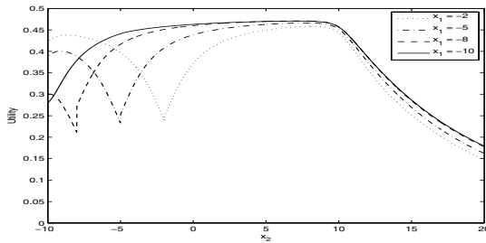
Fig. 5. Single-frequency case; non-cooperating BSs: Utility of BS 2 as a function of its location when we position BS 1 at x_1 where x_1 = -2, -5, -8, -10 .
