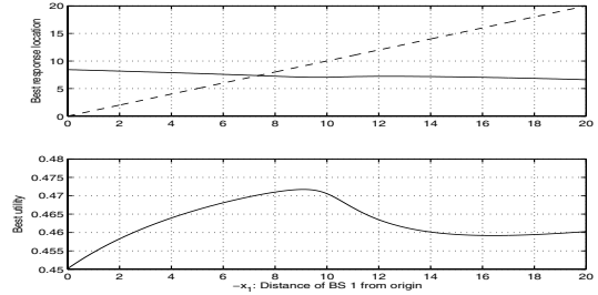
Fig. 6. Single-frequency case; non-cooperating BSs: The top plot shows the best response of BS 2 when BS 1 is at a distance indicated by abscissa to the left of the origin. The bottom plot shows the resulting throughput for BS 2.
