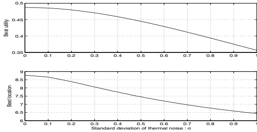
Fig. 4. Single-frequency case; cooperating BSs; symmetric placement of BSs: The top plot shows optimal utility and the bottom plot the optimal symmetric distance from origin for two BSs, as a function of thermal noise standard deviation.
