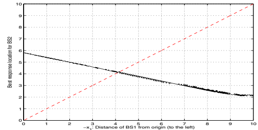
Fig. 7. Two frequencies case; non-cooperating BSs: The best response of BS 2 when BS 1 is at a distance indicated by abscissa to the left of the origin. A positive best response indicates a location on the other side of BS 1.
