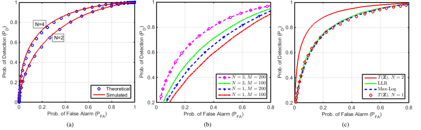
Fig. 1. Receiver operating characteristic (ROC) plot for comparing (a) theoretical and simulated performance of the detector in (14) with K = 12 sensors, M = 250 antennas, N \in \{2, 4\} and SNR p_u = -18 dB. (b) proposed detector in (14) for M \in \{100, 200\} antennas, K = 12 sensors, N \in \{1, 3\} and at SNR p_u = -18 dB. (c) Max-Log and LLR detectors with the proposed detector (14) for M = 250 antennas, K = 12 sensors, N = 1 and at SNR p_u = -18 dB.
