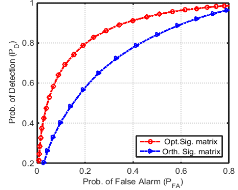
Fig. 2. ROC plot for comparing detector T(\mathbf{Z}) with orthogonal and optimized signaling matrix obtained in Section IV, for a WSN with K = 12 sensors, N = 2 , M = 250 and SNR p_u = -18 dB.
