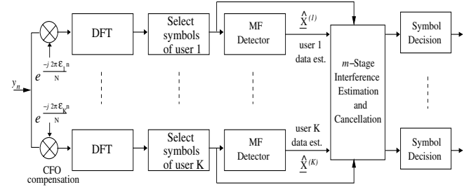
Fig. 4. PIC receiver for cancellation of interferences due to CFOs and TOs in uplink OFDMA without cyclic prefix.
