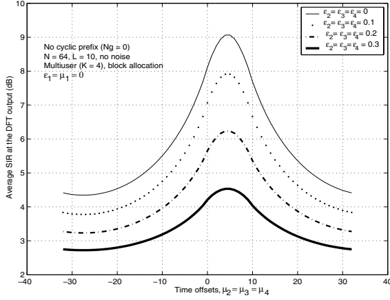
Fig. 3. Average SIR at the DFT output in multiuser uplink OFDMA with CFOs and TOs, and without cyclic prefix ( N_g = 0 ). K = 4 , N = 64 , block allocation of subcarriers, L = 10 , \epsilon_1 = \mu_1 = 0 , \epsilon_2 = \epsilon_3 = \epsilon_4 , \mu_2 = \mu_3 = \mu_4 , no noise.
