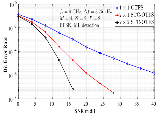
Fig. 4: BER performance of i ) 1 \times 1 OTFS, ii ) 2 \times 1 STC-OTFS, and iii ) 2 \times 2 STC-OTFS for M = 4, N = 2 .
